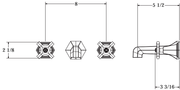
Cross Handles
