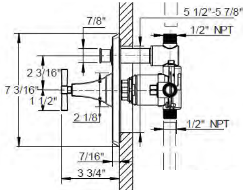
Cross Handle
