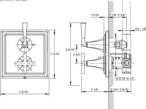
Cross Handle
