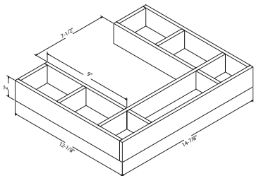
Top Drawer 7 compartments Size: 14-7/8" W x 12-1/8" D x 2" H US-PROORTANT $239
