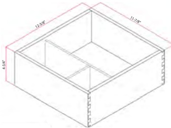
Base Drawer 3 compartments Size: 12-3/8" W x 11-7/8" D x 4-3/4" H US-PROORGB3ANT $199.00
