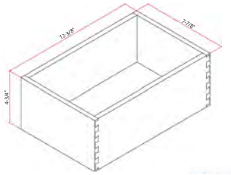
Base Drawer 1 compartment Size: 12-3/8" W x 7-7/8" D x 4-3/4" H US-PROORGB1ANT $139.00
