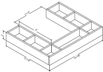
Top Drawer 7 compartments Size: 14-7/8" W x 12-1/8" D x 2" H US-PROORTANT $199.00
