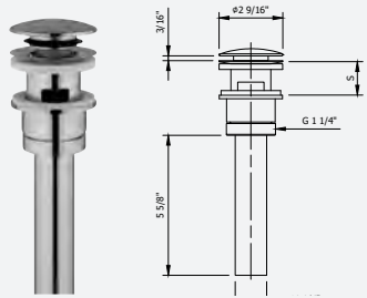
PUSH DRAIN ASSEMBLY INCLUDED
