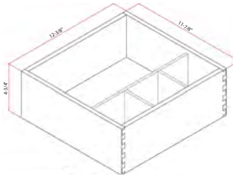
Base Drawer 4 compartments Size: 12-3/8" W x 11-7/8" D x 4-3/4" H US-PROORGB4ANT $219.00
