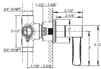
With DIV-RGH, 2 function diverter
